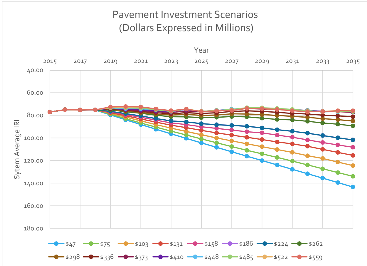
FIGURE 16 – SAMPLE PAVEMENT MODEL RESULTS THAT FEED THE TRADEOFF HUB.
