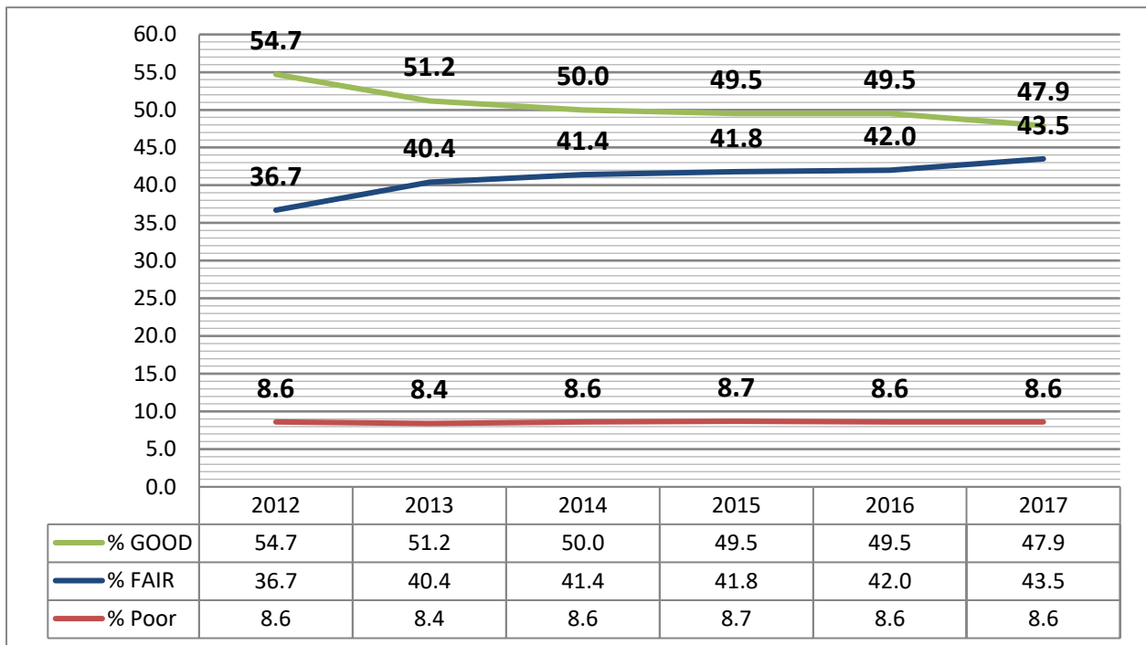
Figure 4.6 Historical Percentage of Good, Fair and Poor NHS Bridges, Excluding Local NHS, by Deck Area
