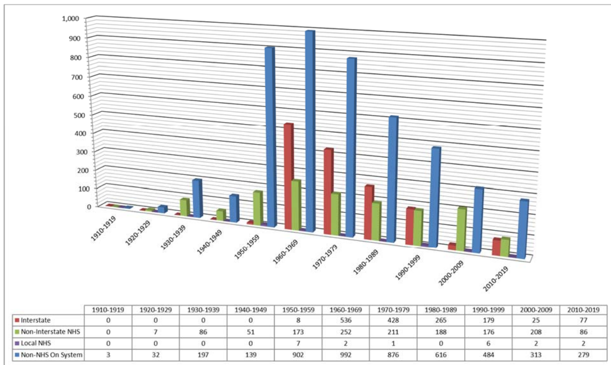
Figure 3.7 Count of Bridges Built By Decade (State Maintained)
