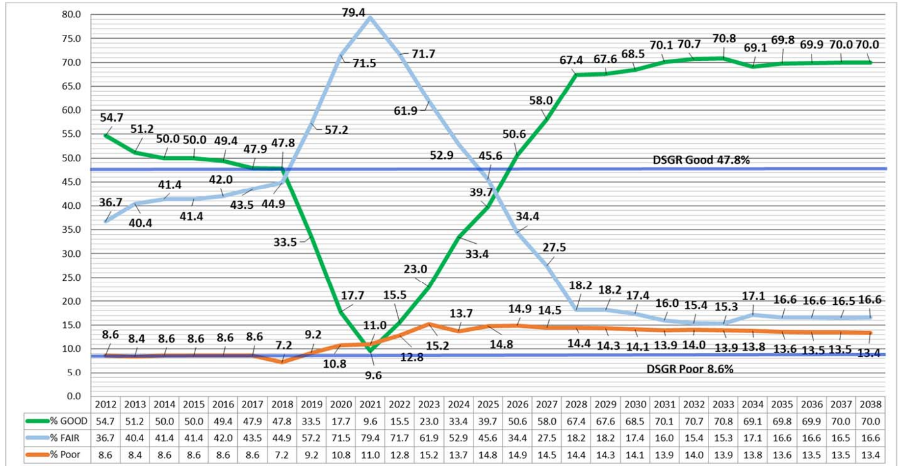
Figure 5.4 Good, Fair & Poor Conditions for Historical & Forecasted NHS Bridge (Excluding Local NHS Bridges)
