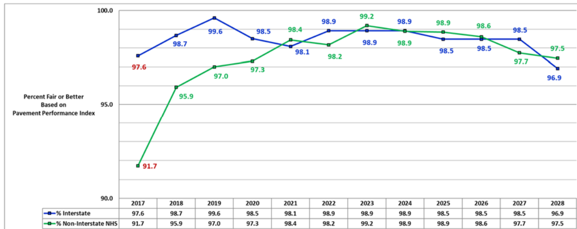
Figure 5.1 Good & Fair Projections by Pavement Condition Index
