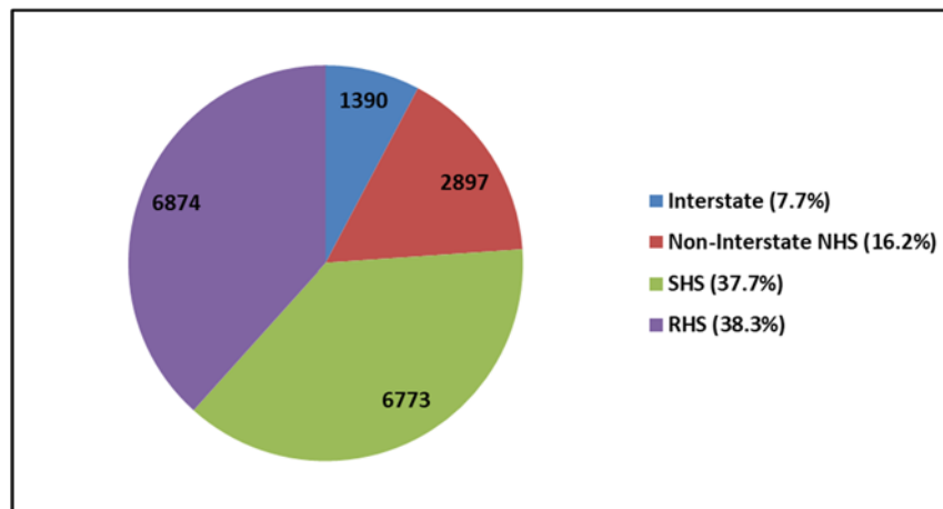
Figure 3.1 Percent PMS Analysis Lane-Miles by Asset Class
