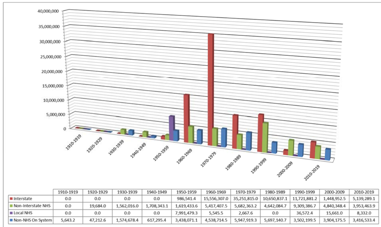
Figure 3.8 Deck Area of Bridges Built By Decade (State Maintained)
