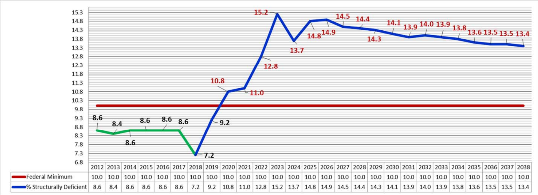
Figure 5.3 SD Condition for Historical (green) & Forecasted (blue) NHS Bridge (based on deck area) (Excluding Local NHS Bridges)
